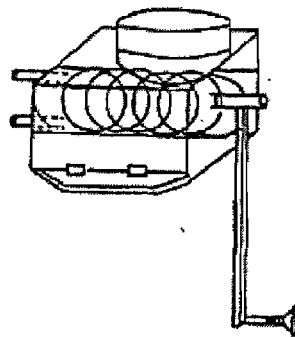
Fig. 2.2 Hand Operated Briquetting Machine
