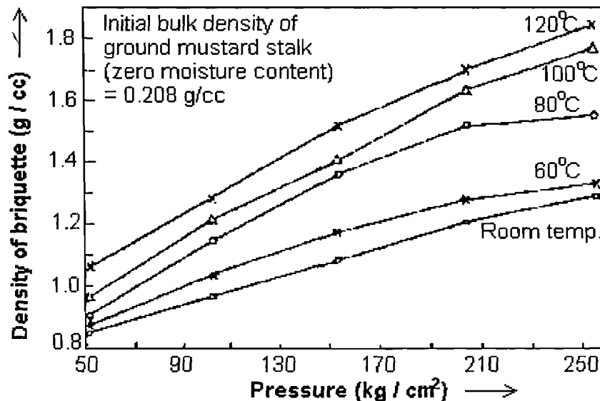
Fig. 4.5 Variation of density with pressure at different temperatures for mustard stalk
