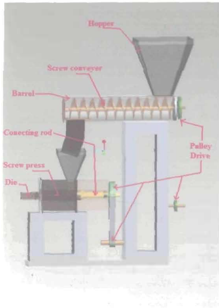
Plate 3.9 Components of screw press briquetting machine
