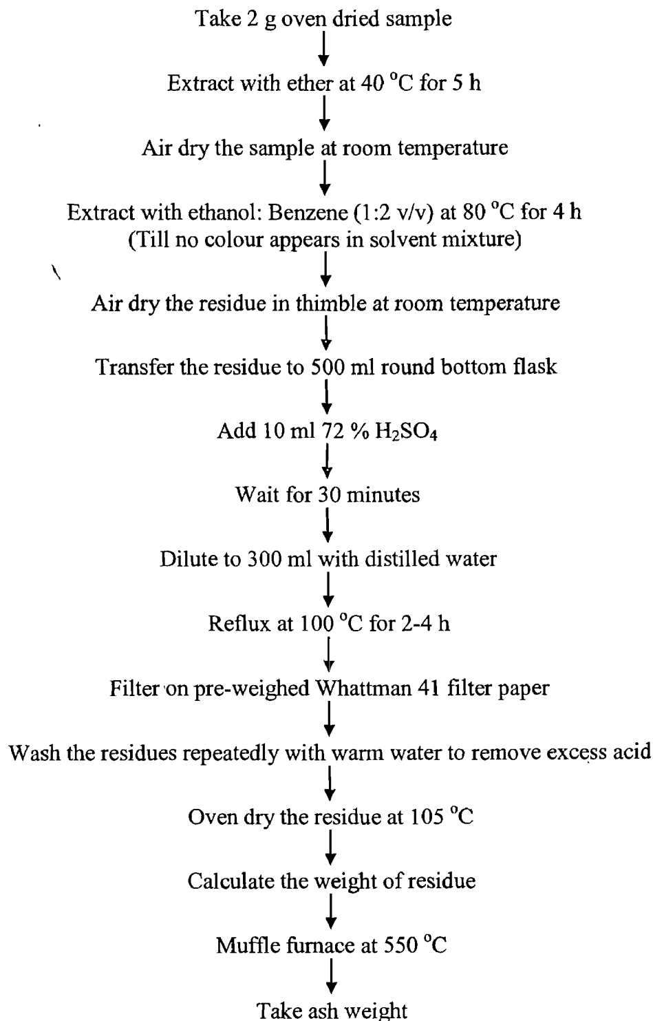
Fig. 3.1 Flow Chart for Quantification of Lignin
