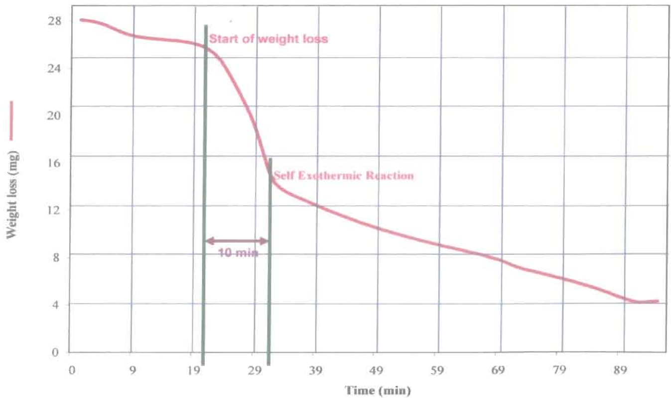
Fig. 4.4 Weight loss of mustard stalk sample with time
