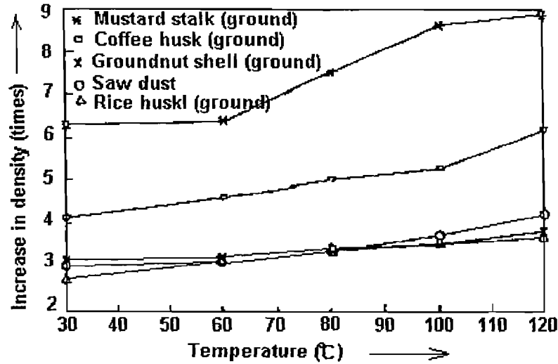
Fig. 4.6 Variation in density with temperature for different materials
