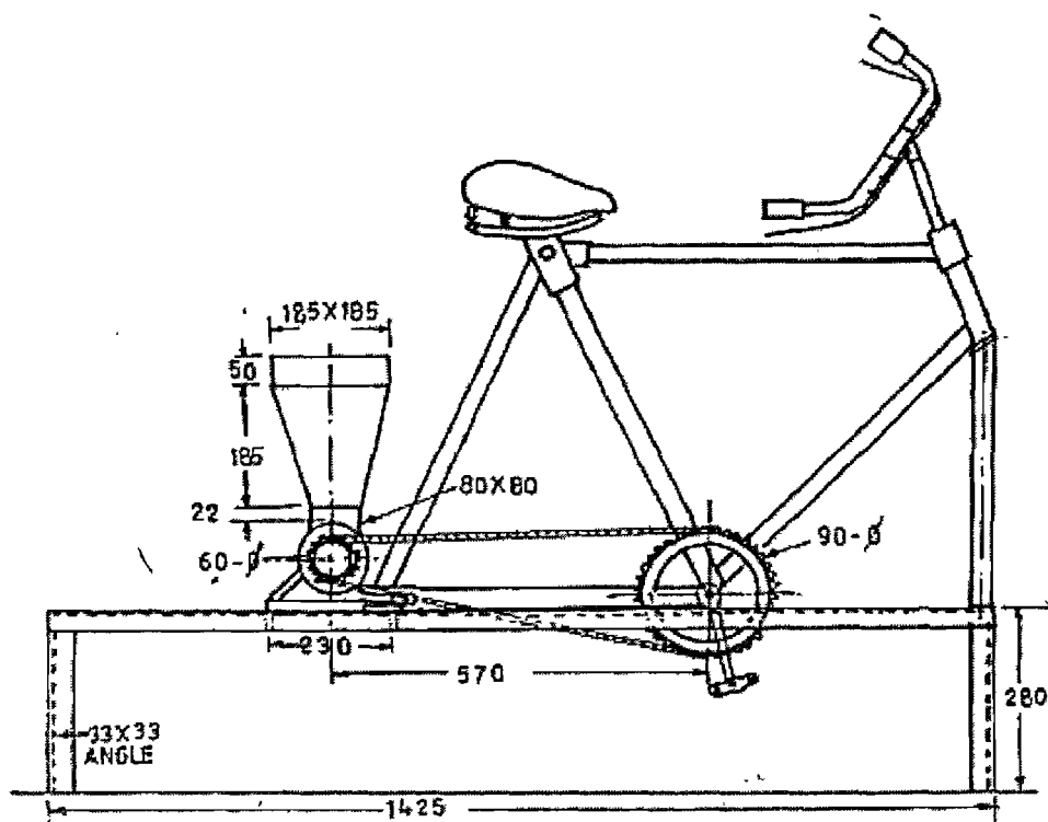
Fig. 2.3 Pedal Operated Briquetting Machine
