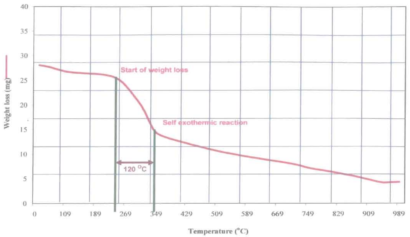
Fig. 4.3 Weight loss of mustard stalk sample with temperature
