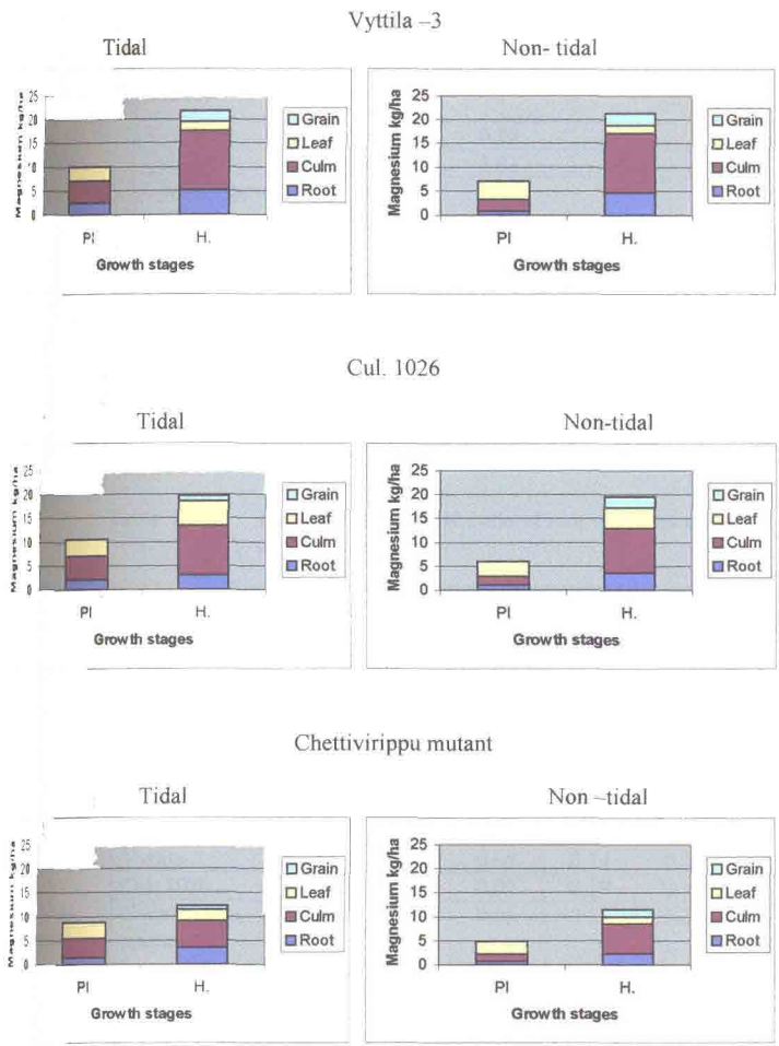
Fig. 13: Effect of tidal regimes on partitioning of Magnesium in rice varieties (kg ha -1 ) -2000
