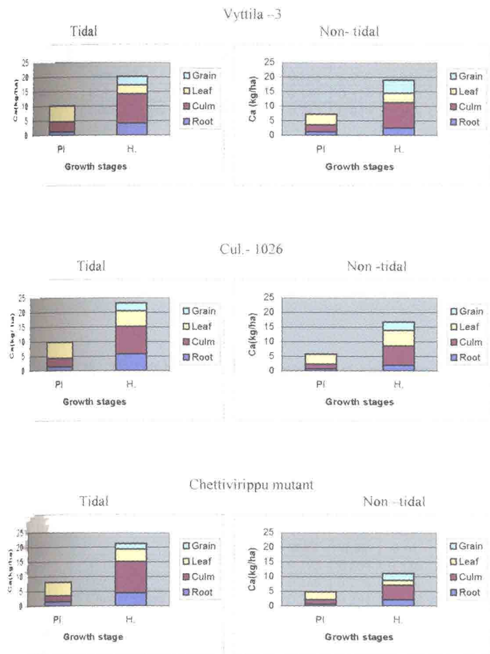
Fig 12 Effect of tidal regimes on partitioning of calcium in rice varieties (kg/ha -1 )-2000
