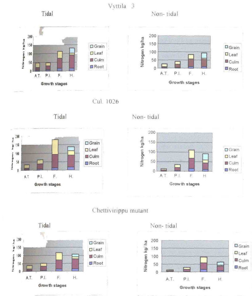
Fig.7 Effect of tidal regimes on partitioning of Nitrogen in rice varieties ( \text{kg ha}^{-1} ) - 2000
