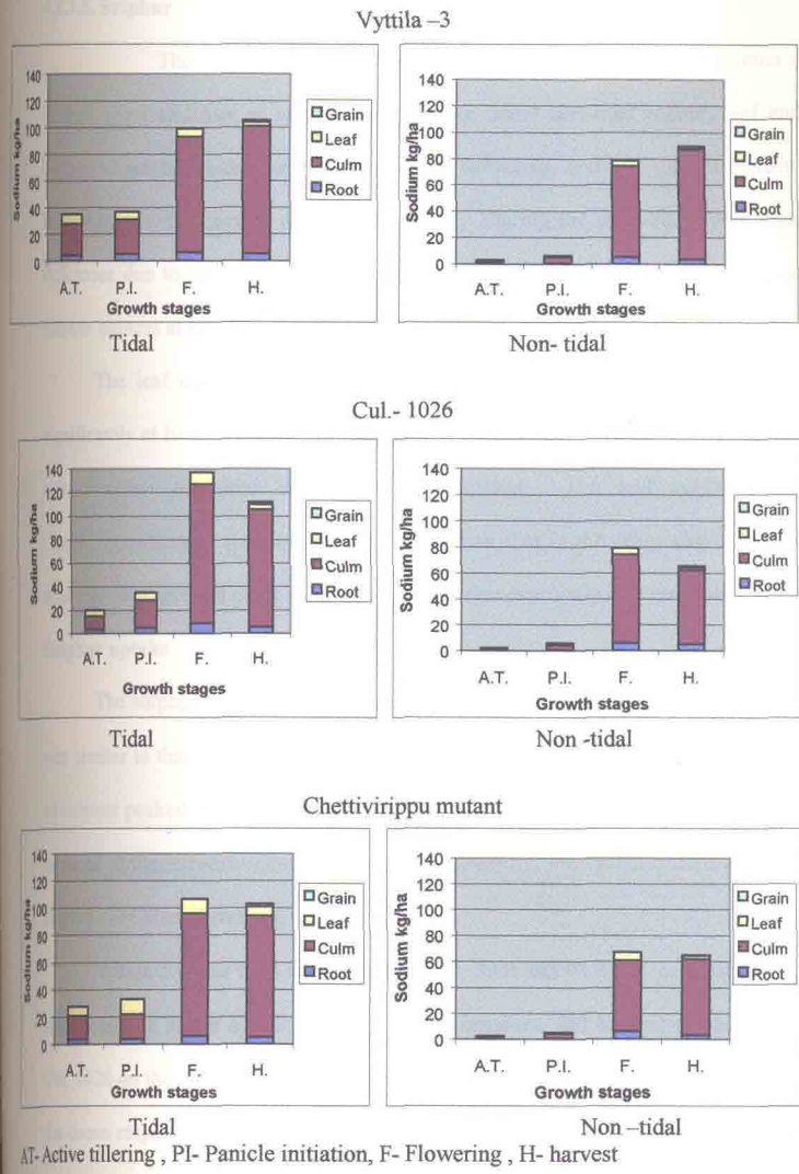
Fig 10. Effect of tidal regimes on partitioning of Sodium in rice varieties ( \text{kg ha}^{-1} )-2000
