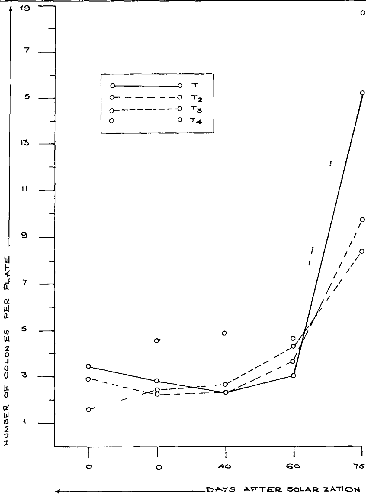
FIG 8 EFFECT OF SOLARIZATION ON SOIL BACTERIA IN OPEN FIELD
