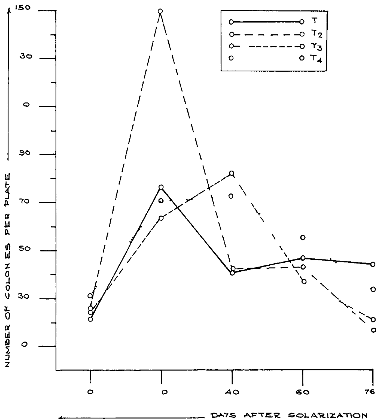
FIG 6 EFFECT OF SOLARIZATION ON SOIL MYCOFLORA IN OPEN FIELD
