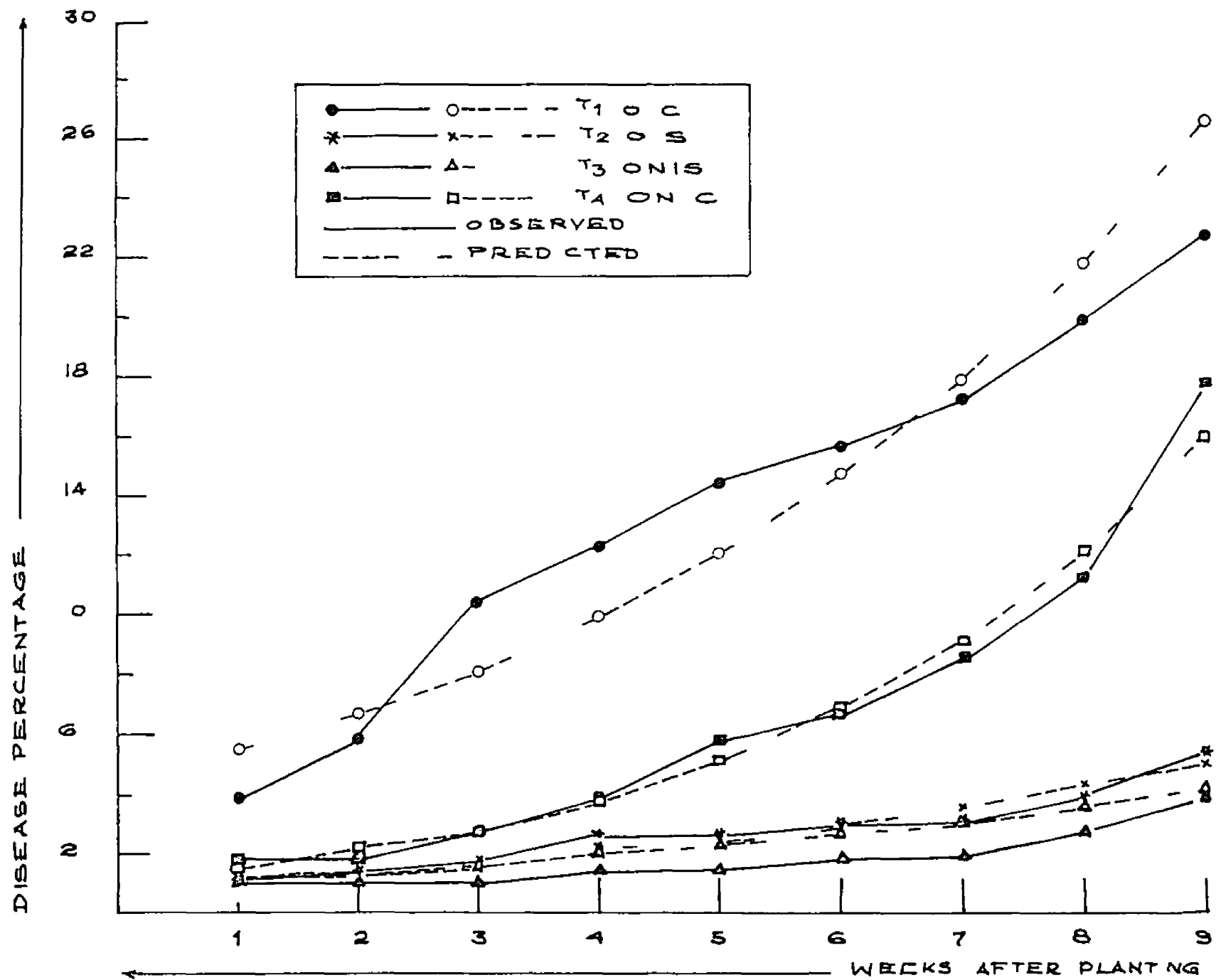
FIG 3 NOCULUM POTENTIAL OF P. solani IN SOILS
