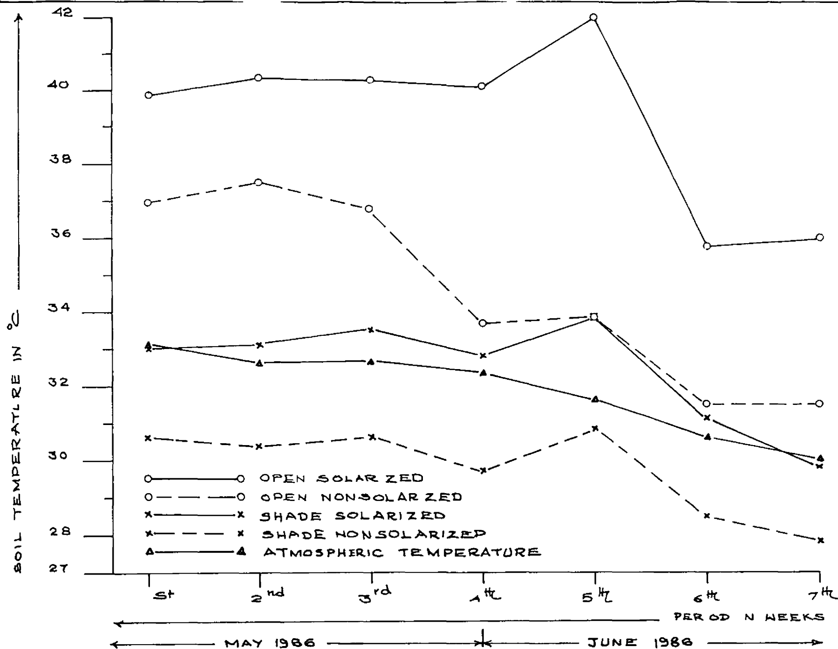
FIG 2 ATMOSPHERIC AND SOIL TEMPERATURE (WEEKLY MEAN) DURING SOIL SOLARIZATION
