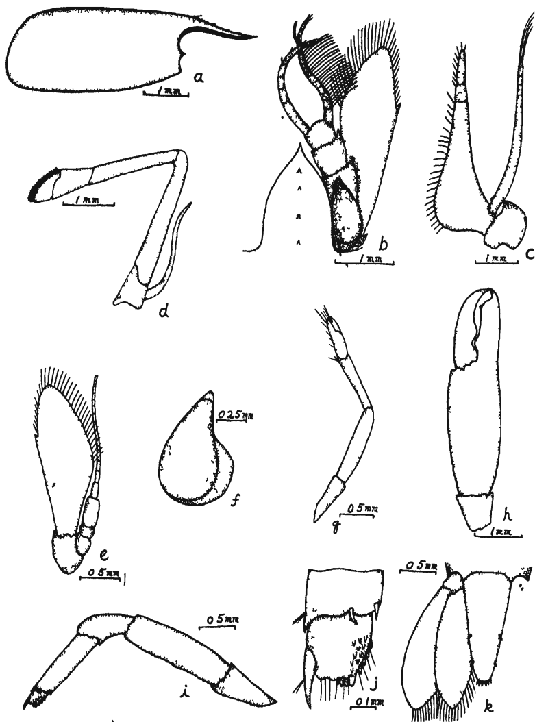
FIGURE 2.—Structural features of Coralhocaris mammillata , new species: a , lateral view of carapace; b , dorsal view of rostrum, eye, antennule, and scale of antenna; c , outer maxilliped; d , second maxilliped; e , basal part of antenna and scale; f , eye; g , first leg; h , wrist and hand of second leg; i , third leg; j , dactylus of third leg; k , telson and uropod
