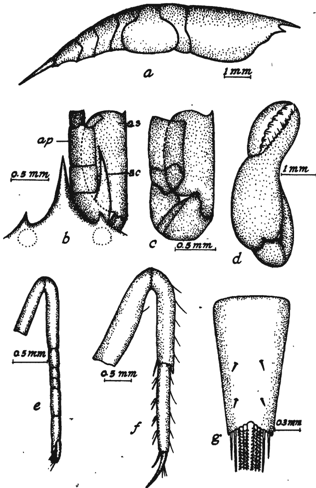
FIGURE 2.— Jousseaukea mauiensis , new species: a , carapace and abdomen from right side; b , frontal region, including antennular peduncle ap , stylocerite, sc , and antennal scale, as ; c , antennal peduncle and scale; d , large (right) cheliped; e , second leg, right side; f , third leg, right side; g , telson.
