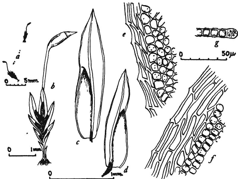
FIGURE 1— Fissidens raiatensis Bartram, new species a two plants, b , moist plant, c , perichaetial leaf d , stem leaf, e , cells and margin of apical blade, f , cells and margin of duplicate blade, g , cross section of leaf margin
