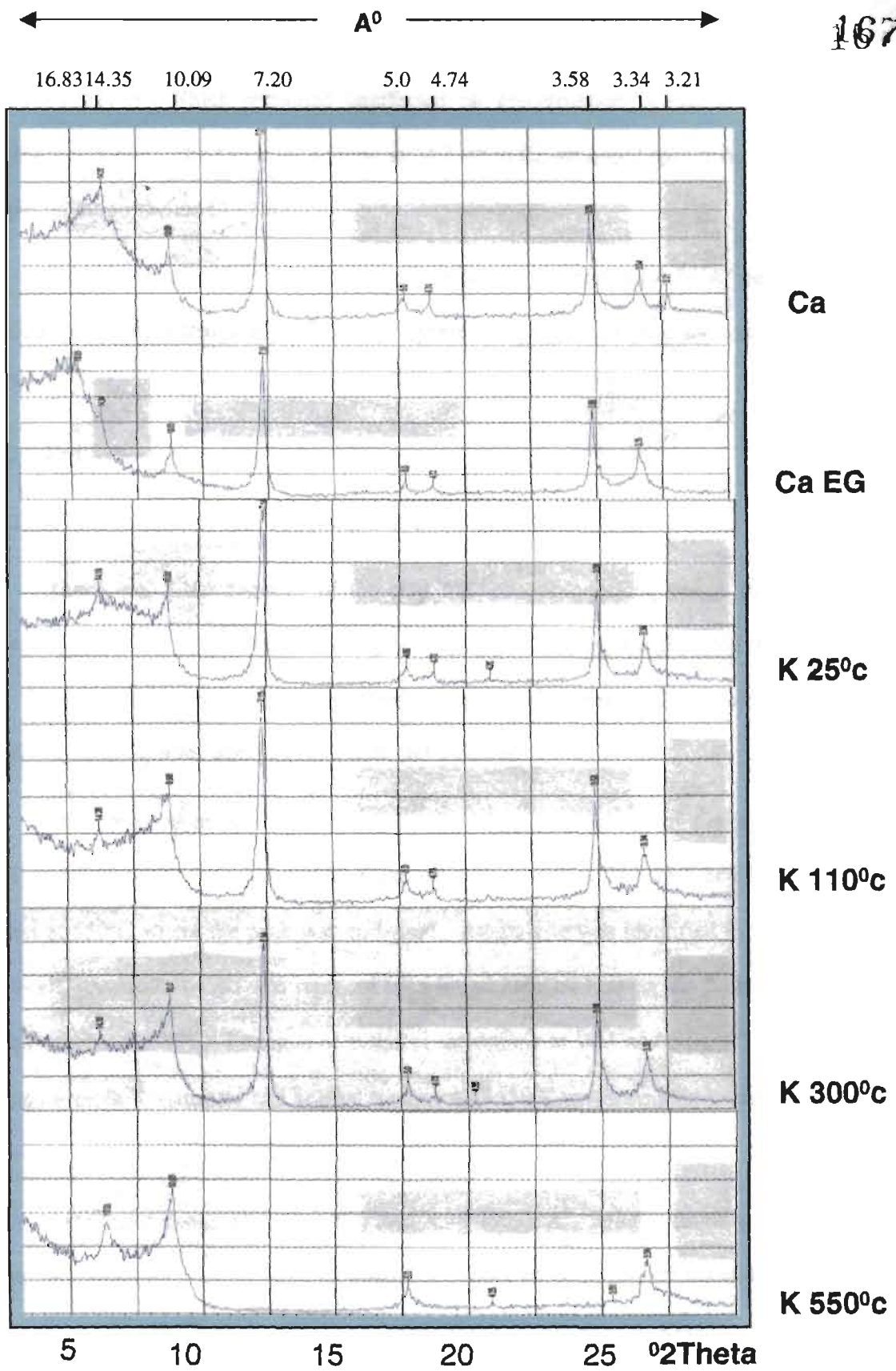
Fig.18 : X-ray diffractograms of clay fraction of soils in Dhaneti - 1 series
