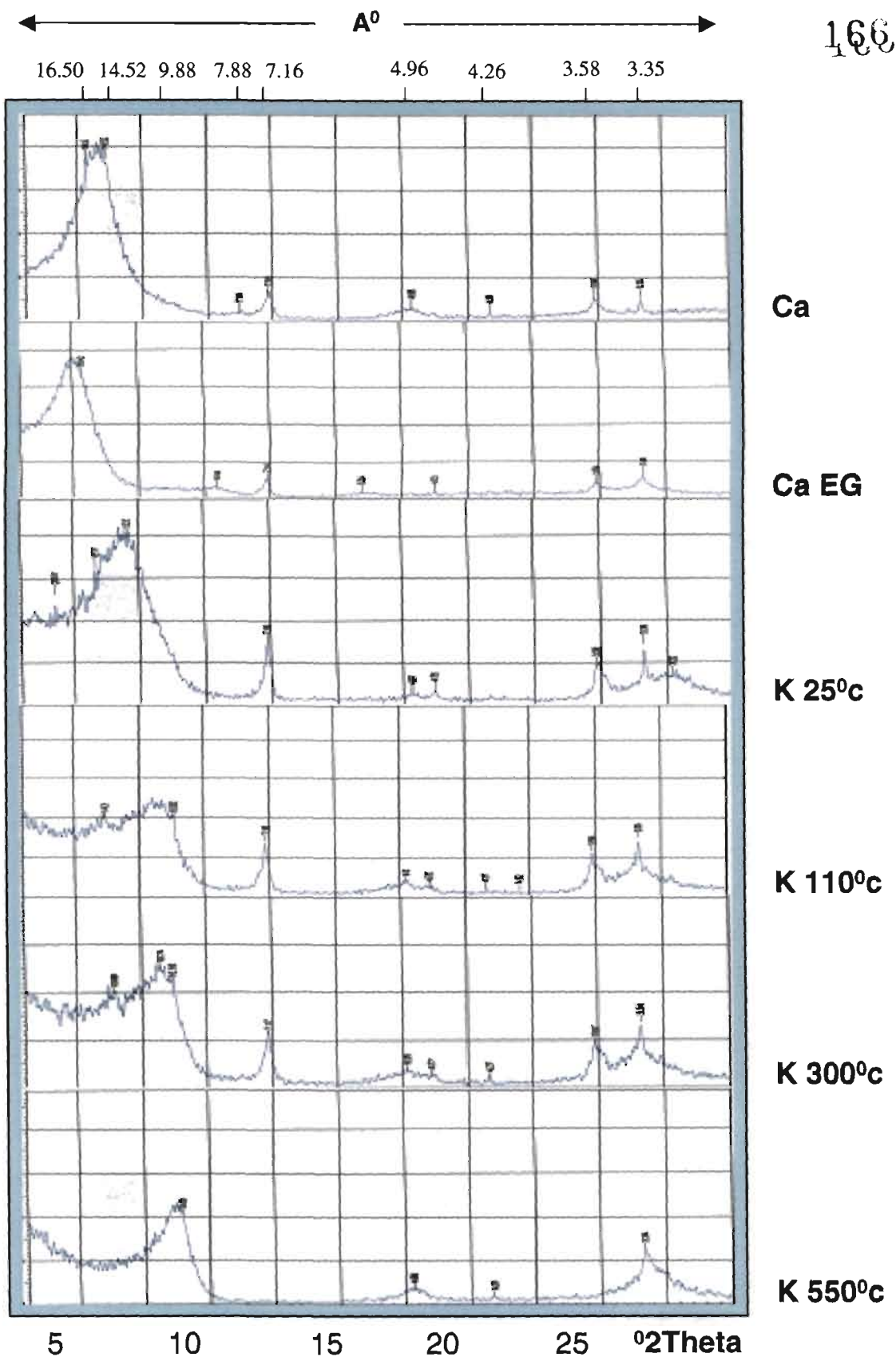
Fig.17 : X-ray diffractograms of clay fraction of soils in Amrutanagar series
