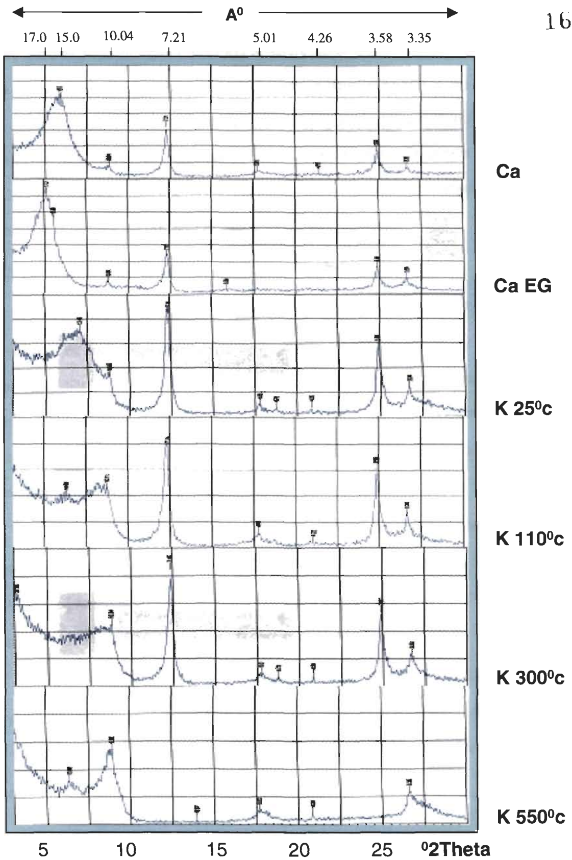
Fig.15 : X-ray diffractograms of clay fraction of soils in Dagala - 1 series
