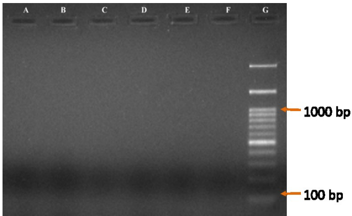
Plate 7 Agarose gel electrophoresis of PCR product from cDNA of Thekken and Karimunda from different developmental stages using RA1 gene primers
