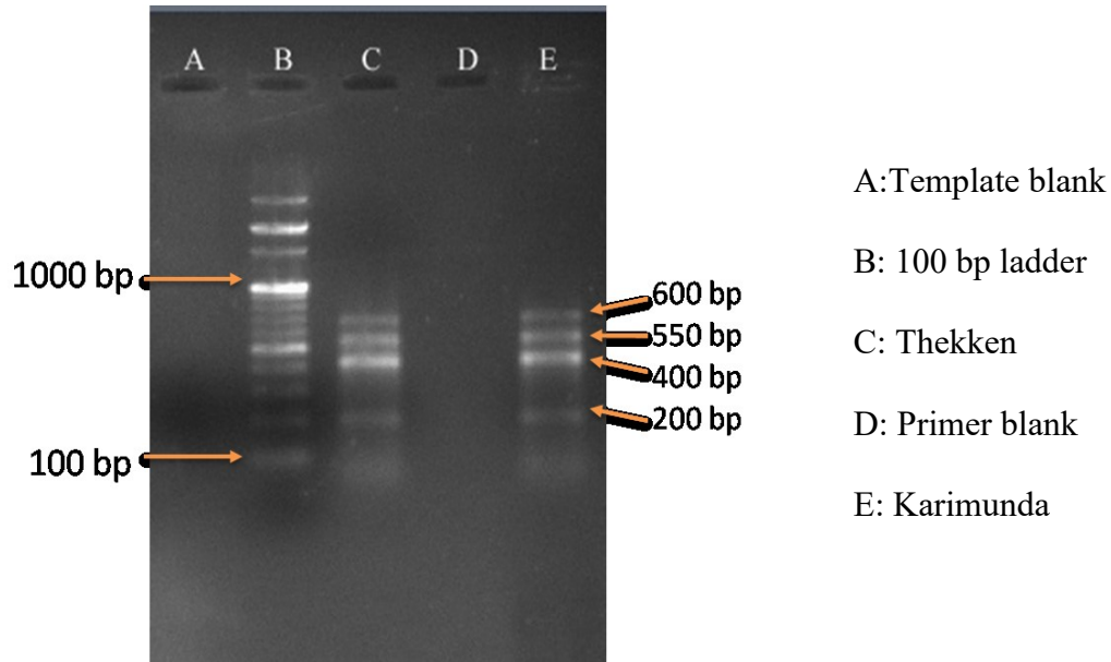
Plate 3 Agarose gel electrophoresis of PCR product from genomic DNA of Thekken and Karimunda using RA1 primers
