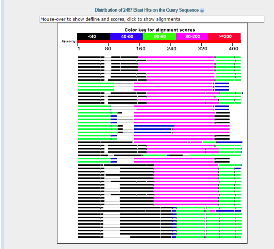
Plate 11a Screenshot showing the result of TBLASTX of sequence obtained with primer RA2R of RA2 gene
