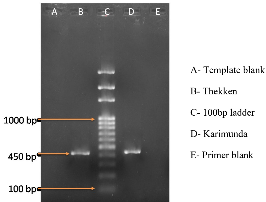
Plate 4 Agarose gel electrophoresis of PCR product from genomic DNA of Thekken and Karimunda using RA2 primers
