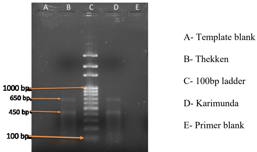
Plate 5 Agarose gel electrophoresis of PCR product from genomic DNA of Thekken and Karimunda using RA3 primers
