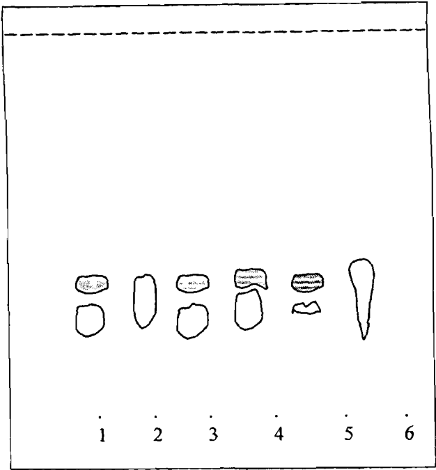
Fig. 4. Colorific pigments from safflower flowers in thin layer chromatogram. Positions 1-5 represent pigments from acetone washing of reddish cellulose. Position 6 represents water-soluble yellow pigment from safflower.
