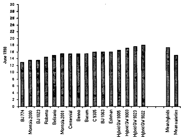
Fig. 1. Date of 50% blooming as a mean of the 2 localities.
