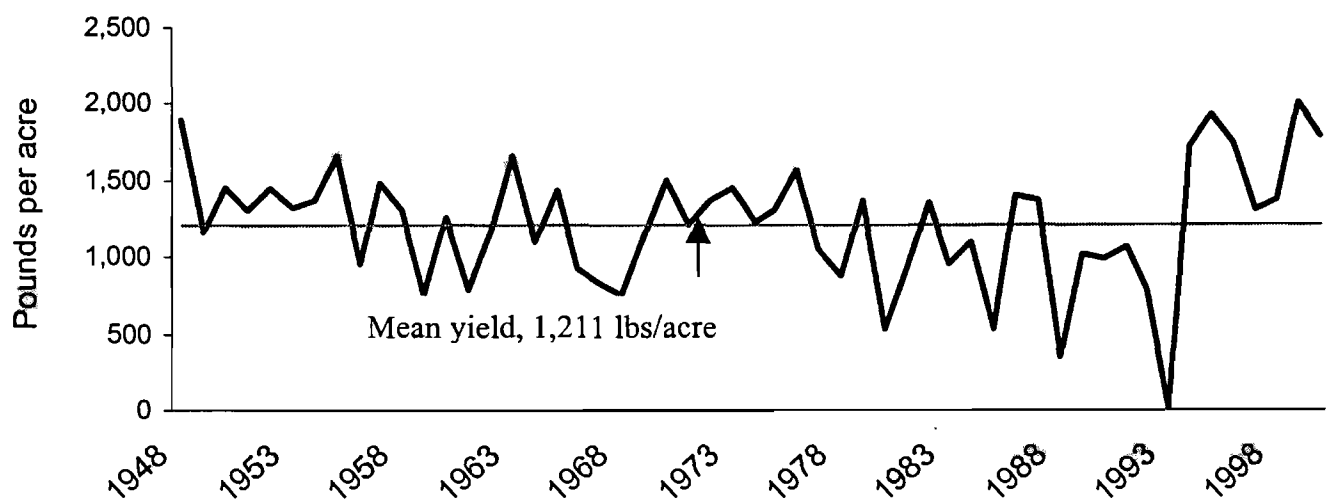
Fig. 2. Montana safflower dryland yield, pounds per acre, 1948-2000.
