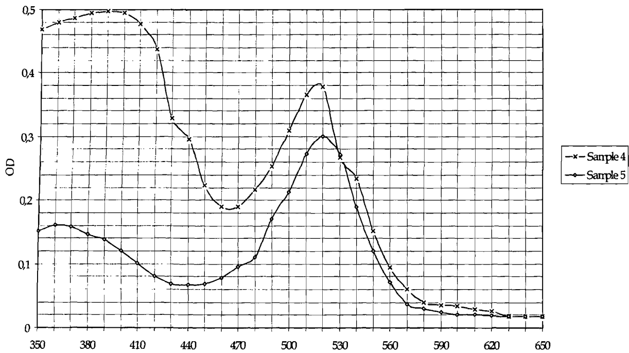
Fig. 2. OD of carthamine of acetone washing of radish cellulose (Sample 4 and 5).
