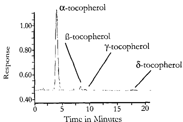
Fig. 2. High Performance Liquid Chromatogram showing peak identification and tocopherol profile of Morlin variety safflower oil.
