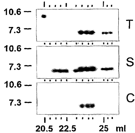
Fig. 3. Detection of trypsin (T), chymotrypsin (C) and subtilisin (S) inhibitors in protein fractions eluted from HPLC-RP (Fig. 2). Proteins were separated by IEF and inhibitors were detected by gelatin replicas method.
