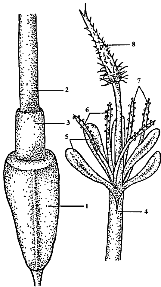
Fig. 1. Morphological structure of the flower and nectar-bearing tissue in the safflower (original).
