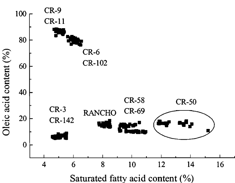
Fig. 1. Scatter plot of saturated fatty acid (palmitic+stearic) content versus oleic acid content in half-seeds of lines with different fatty acid profiles and the cultivar 'Rancho', used as check.
