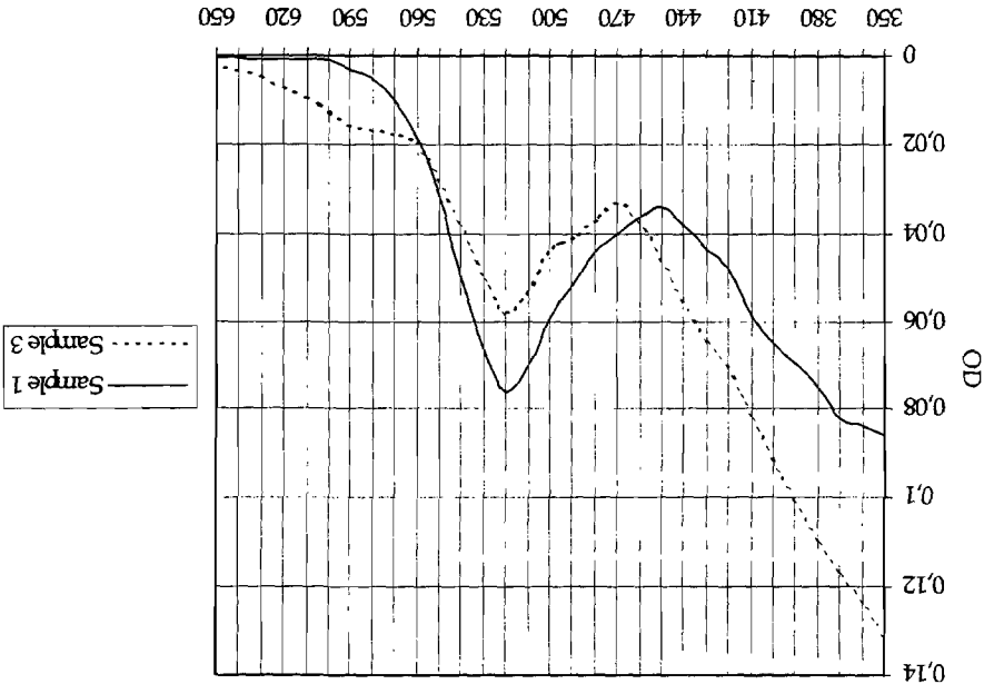
Fig. 1. Optical density (OD) of acetone washing of reddish cellulose (sample 1 and 3.)
