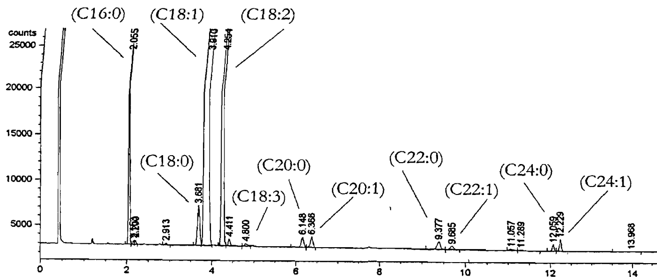
Fig. 1. Gas Liquid Chromatogram showing peak identification and fatty acid profile oil from a high oleic safflower breeding line.
