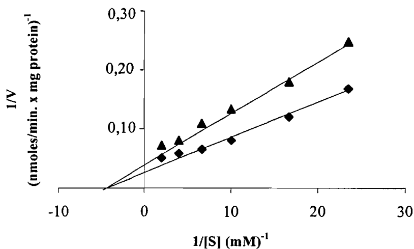
Fig 2. Lineweaver and Burk plot of citrate/malate exchange catalyzed by freshly isolated rat liver mitochondria
