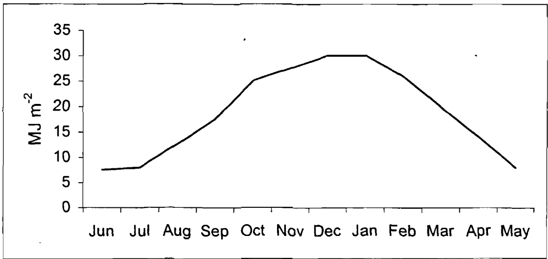
Fig. 3. Average overall radiation at Anguil (36° 30'S 64° W).
