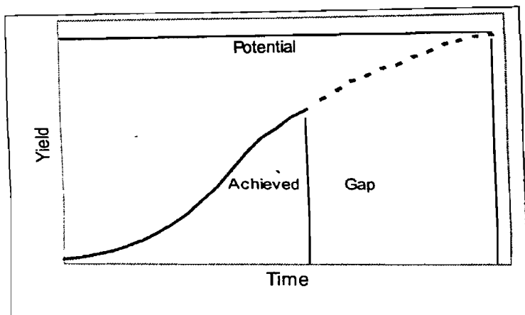
Fig. 3. Growth model for depicting time for realizing yield
