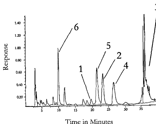
Fig. 3. High Performance Liquid Chromatogram of phenolic glucosides in defatted Morlin variety safflower meal.
