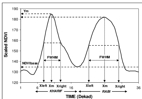
Figure 2. Schematic showing phenology metrics for Kharif and Rabi seasons.
