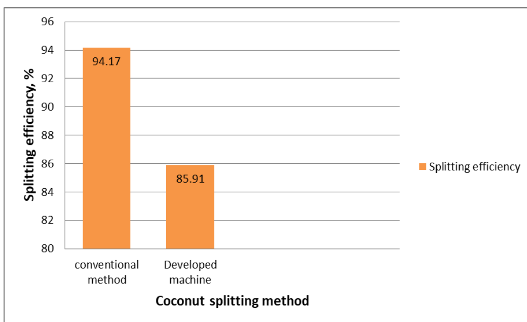
Fig 4.2 Splitting efficiency of two coconut splitting methods
