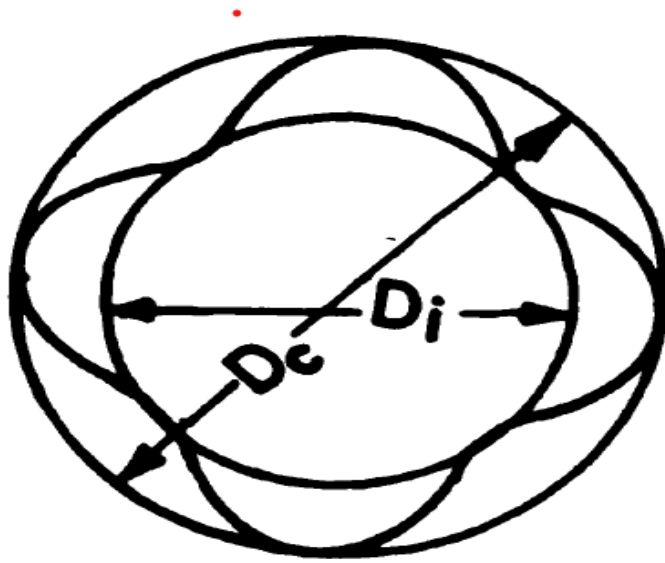
Fig. 3.2 Diagram of smallest circumscribing and largest inscribing circles of a particle
