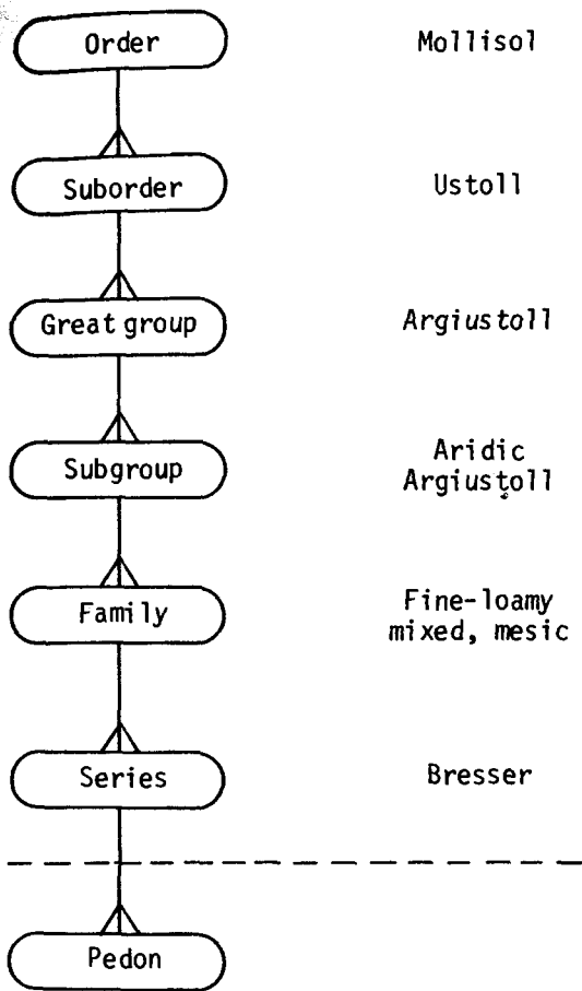
Figure 2. Overview of the hierarchal structure of Soil Taxonomy , a soil classification schema.
