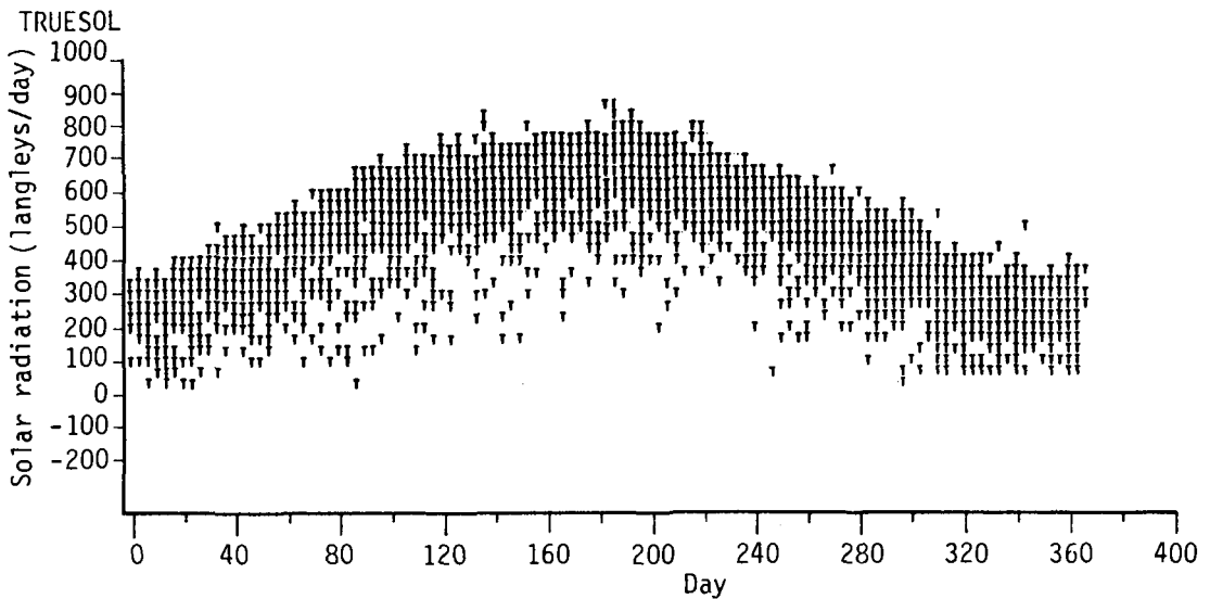
Figure 6. Observed distribution of solar radiation at Oklahoma City, Okla, USA (1971-1972).
