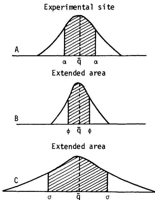
Figure 4. Illustration of three areas with identical mean ( \bar{q} ) and different standard deviations.
