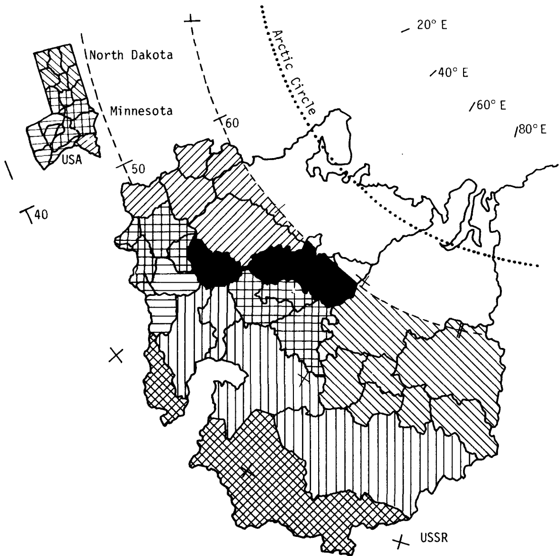
Figure 9. Areas with expected similar crop response in the USSR and in North Dakota and Minnesota, USA, as determined by a clustering technique. Similar hatched areas have similar defined environmental characteristics. (Source: French et al. 1982.)
