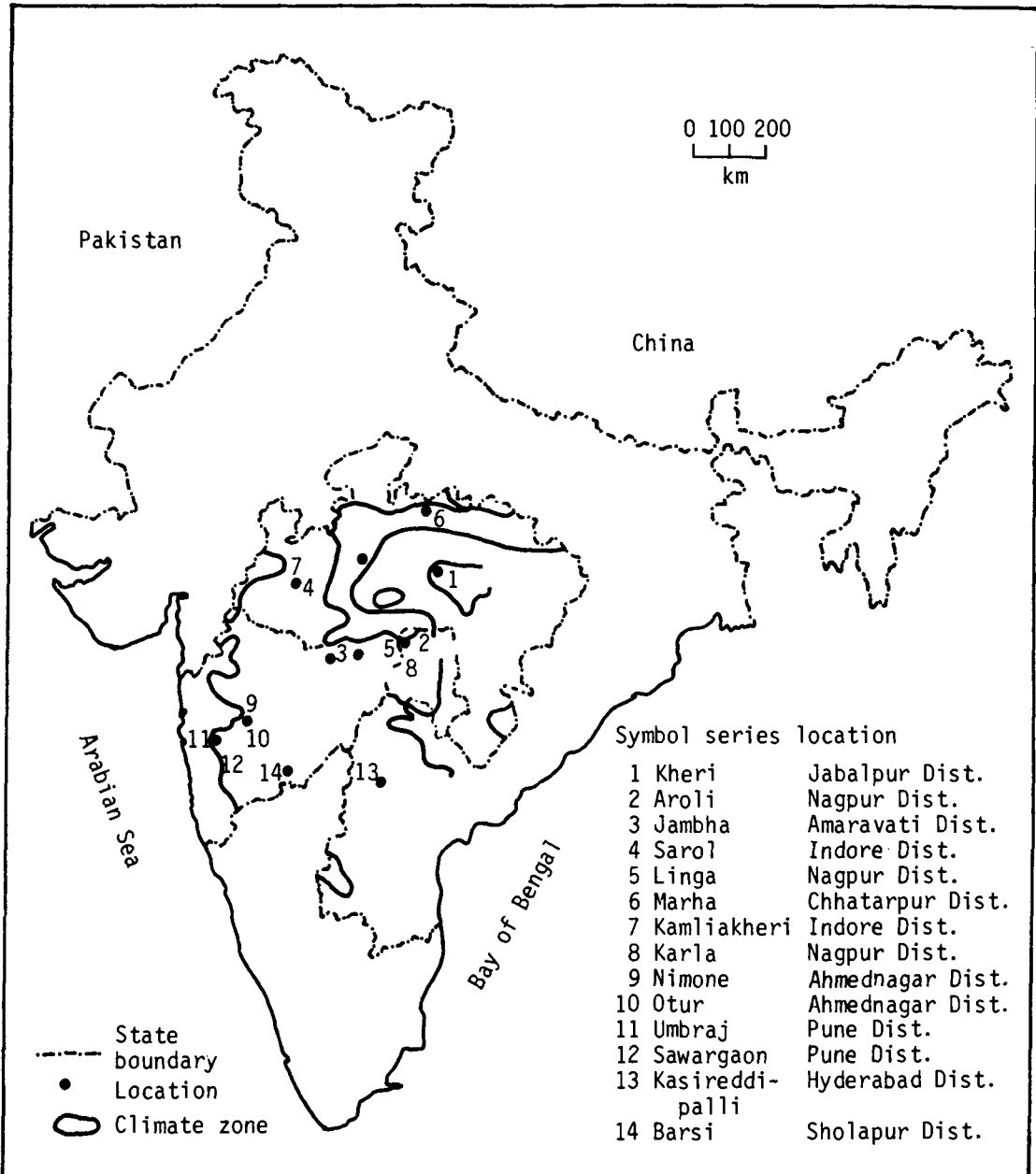
Figure 2. Benchmark Soils Project area and environs in central peninsular India. A. Humid, hot, with large summer water deficiency; B. Moist, subhumid, hot with large summer surplus; C. Dry, subhumid, hot, with large summer surplus; D. Dry subhumid, with moderate summer surplus; E. Semi-arid, hot, with moderate summer surplus; F. Semi-arid, hot, with little or no surplus; G. Arid, hot, with little or no surplus.
