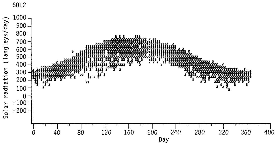
Figure 7. Seasonal distribution of simulated solar radiation (after Hodges et al. 1983) at Oklahoma City, Okla, USA (1971-1972).
