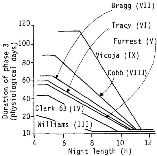
Figure 3. Duration of phase 3 of development in seven soybean cultivars, as a function of night length. (Source: Mishoe et al. 1983.)
