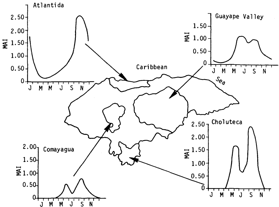
Figure 2. Moisture availability index (MAI) for four areas in Honduras (adapted from Hargreaves 1981).
