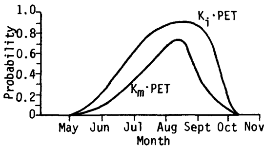
Figure 3. Probability of precipitation exceeding the maximum crop water requirement ( K_m \cdot PET ) and the threshold crop water requirement ( K_i \cdot PET ) (adapted from Gommès and Houssian 1982).
