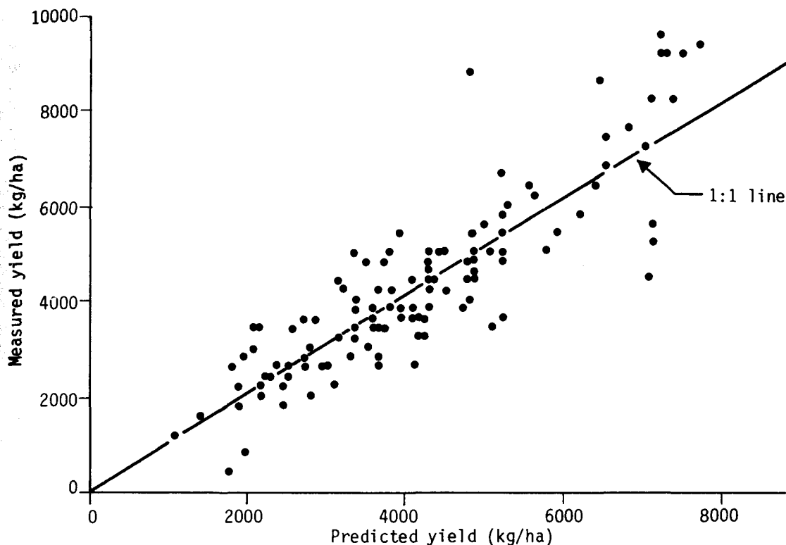
Figure 1. Preliminary test results from comparisons of measured and CERES-simulated growth, development, and yield of wheat.
