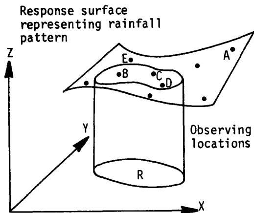
Figure 1. Illustration of the space domain of crop region R represented by station B, C, and D. A is an experimental site, the technology of which is to be transferred to R; E is a station outside the crop region.
