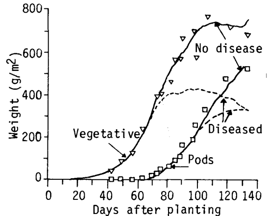
Figure 10. Experimental data of vegetative ( \Delta ) and pod ( \square ) dry weights for disease-free groundnut and for an assumed incidence of Cercospora leaf-spot disease were obtained with the SOYGRO-converted groundnut growth model. (Source: Boote et al. 1983.)
