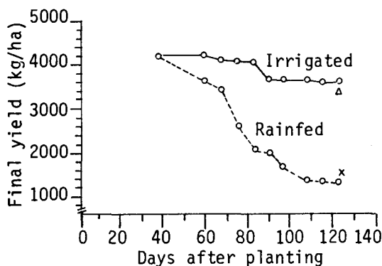
Figure 9. Weekly yield predictions made by SOYGRO for two treatments in an experiment conducted in Gainesville, Fla, in 1981 by K. J. Boote, J. M. Bennett, L. C. Hammond, and J. W. Jones (unpublished). Yields measured at the end of the season are denoted by \Delta (irrigated treatment) and by X (rainfed treatment).
