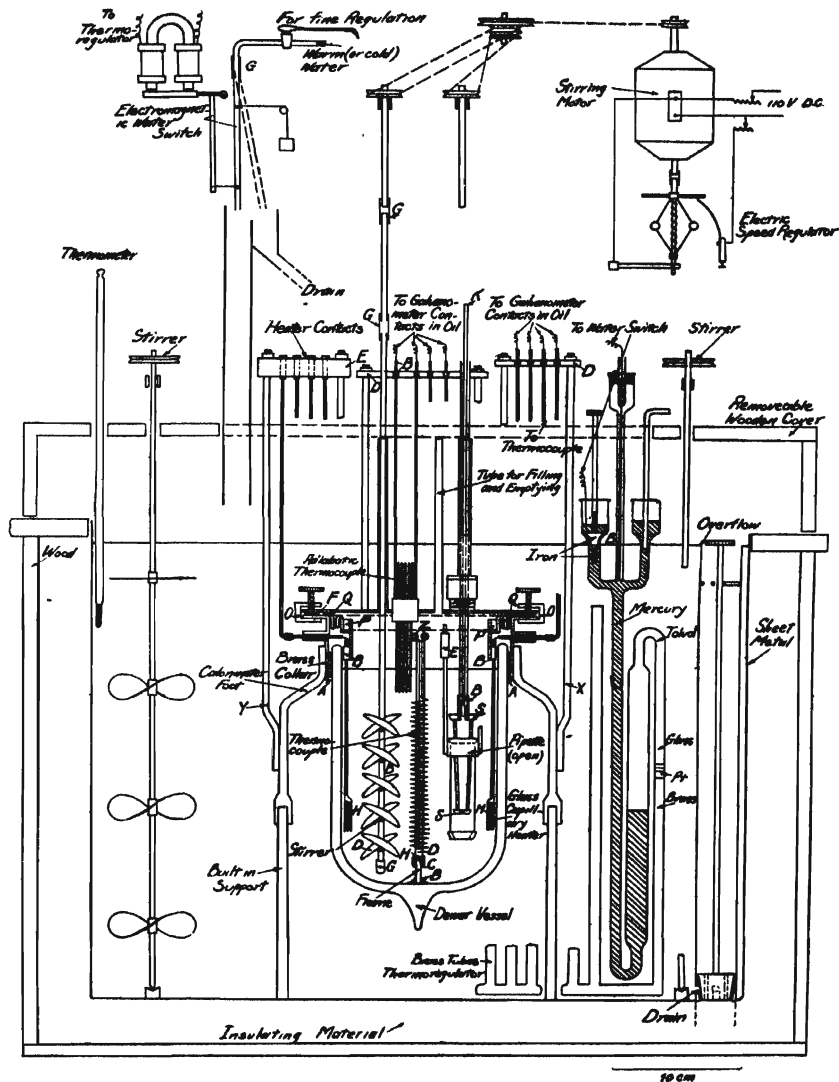
FIG. 3. ADIABATIC DIFFERENTIAL CALORIMETER
