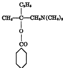
Stovaine
