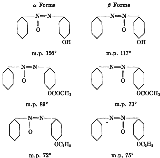
FIG. 7. \alpha AND \beta FORMS OF BENZENEAZOXY- p -PHENOL AND SOME OF ITS DERIVATIVES
