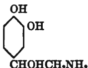
Norepinephrine
