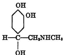
Epinephrine
