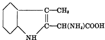
Skatoleaminoacetic acid
