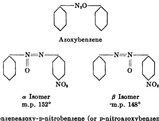
FIG. 1. AZOXYBENZENE AND ISOMERS OF BENZENEAZOXY- p -NITROBENZENE
