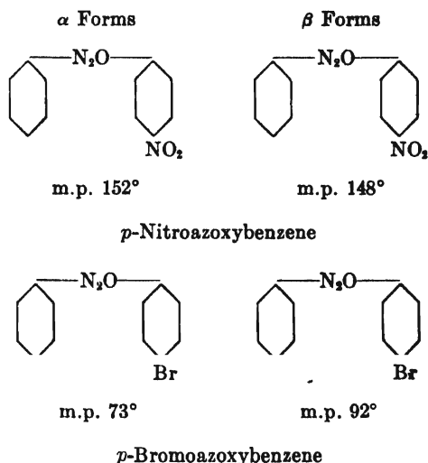
FIG. 2. ISOMERIC FORMS OF p -NITROAZOXYBENZENE AND p -BROMOAZOXYBENZENE
