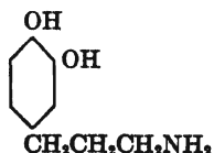
XIX
