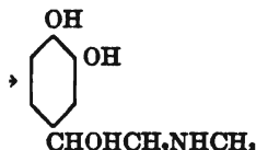
Epinephrine
