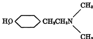
Hordenine
