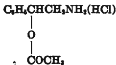
XXIII
