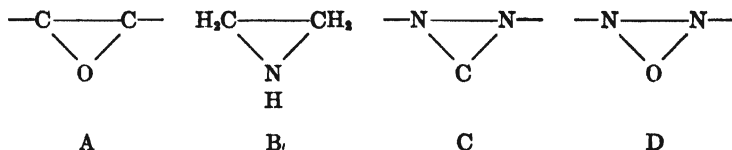
FIG. 8. CERTAIN THREE-MEMBERED RINGS
