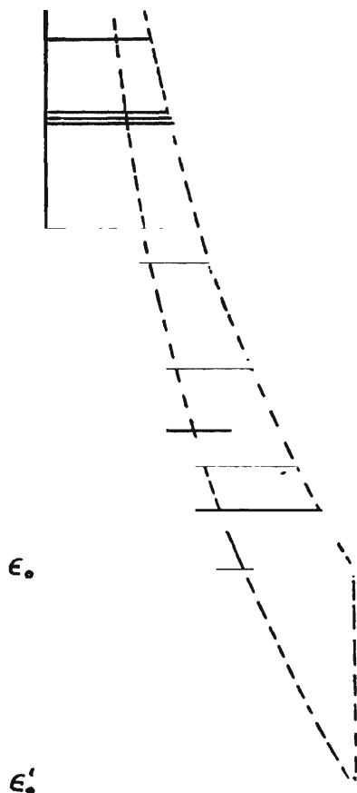
FIG. 3. GRAPHICAL REPRESENTATION OF THE PARTITION FUNCTION
