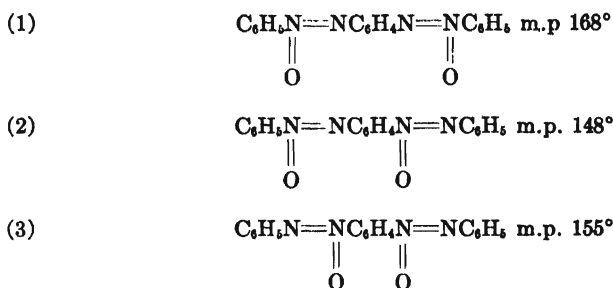
FIG. 9. THE THREE POSSIBLE ISOMERIC FORMS OF BISAZOXYBENZENE
