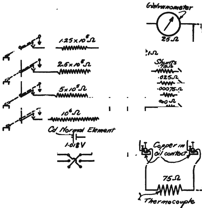
FIG. 5. DIAGRAM OF GALVANOMETER CONNECTION TO THERMOCOUPLE
