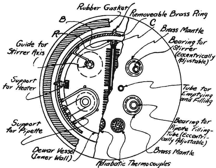
FIG. 2. TOP VIEW OF CALORIMETER VESSEL
