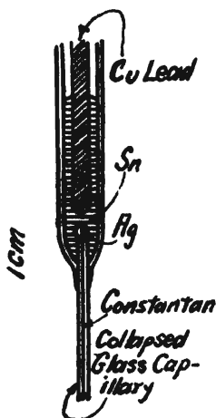
FIG. 4. DETAIL OF CAPILLARY HEATER
