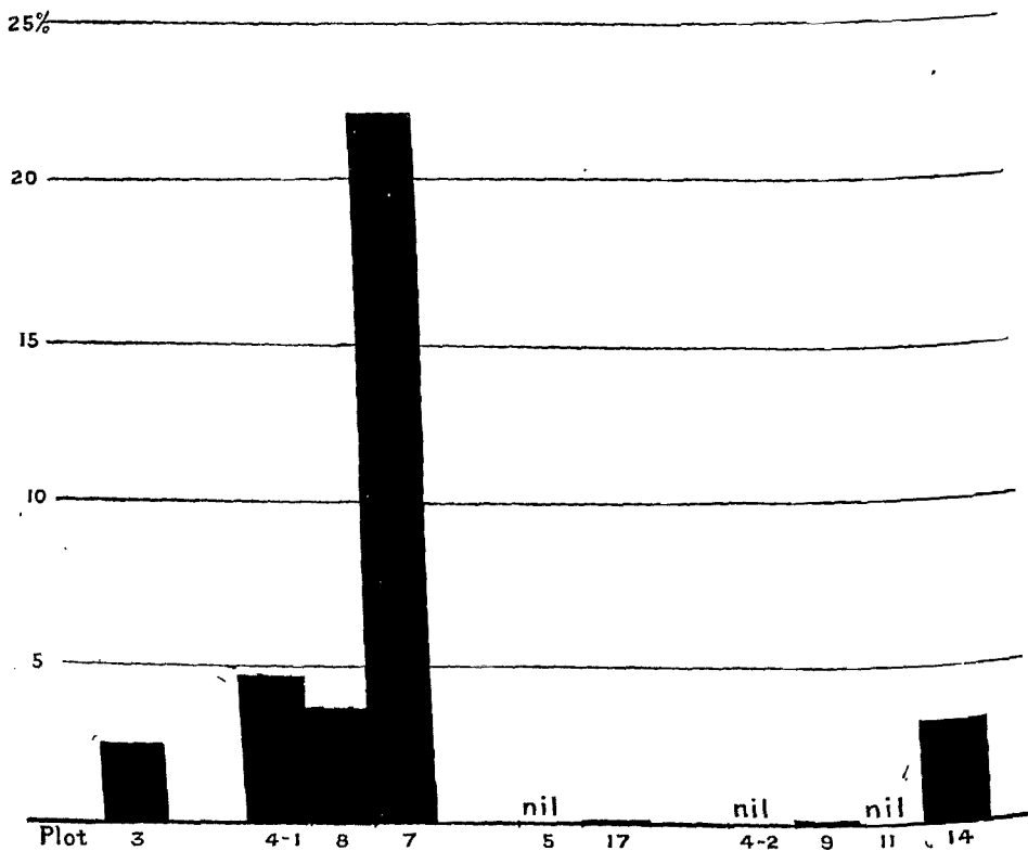
FIG. 88.—Percentage of Lathyrus pratensis in the Herbage of the Grass Plots. First Crop, Season 1903.
