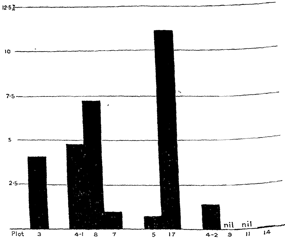
FIG. 39.—Percentage of Centaurea nigra in the Herbage of the Grass Plots. First Crop, Season 1903.
