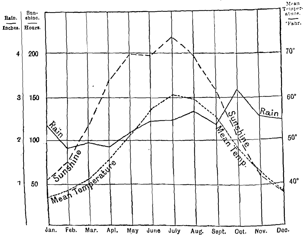
FIG. 1.—Rainfall: Average of 60 years (1853-1912). Sunshine: Average of 20 years (1892, 1893, and 1895-1912). Mean Temperature: Average of 35 years (1878-1912).
