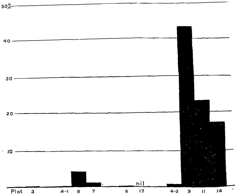
FIG. 35.—Percentage of Arrhenatherum avenaceum in the Herbage of the Grass Plots. First Crop, Season 1903.
