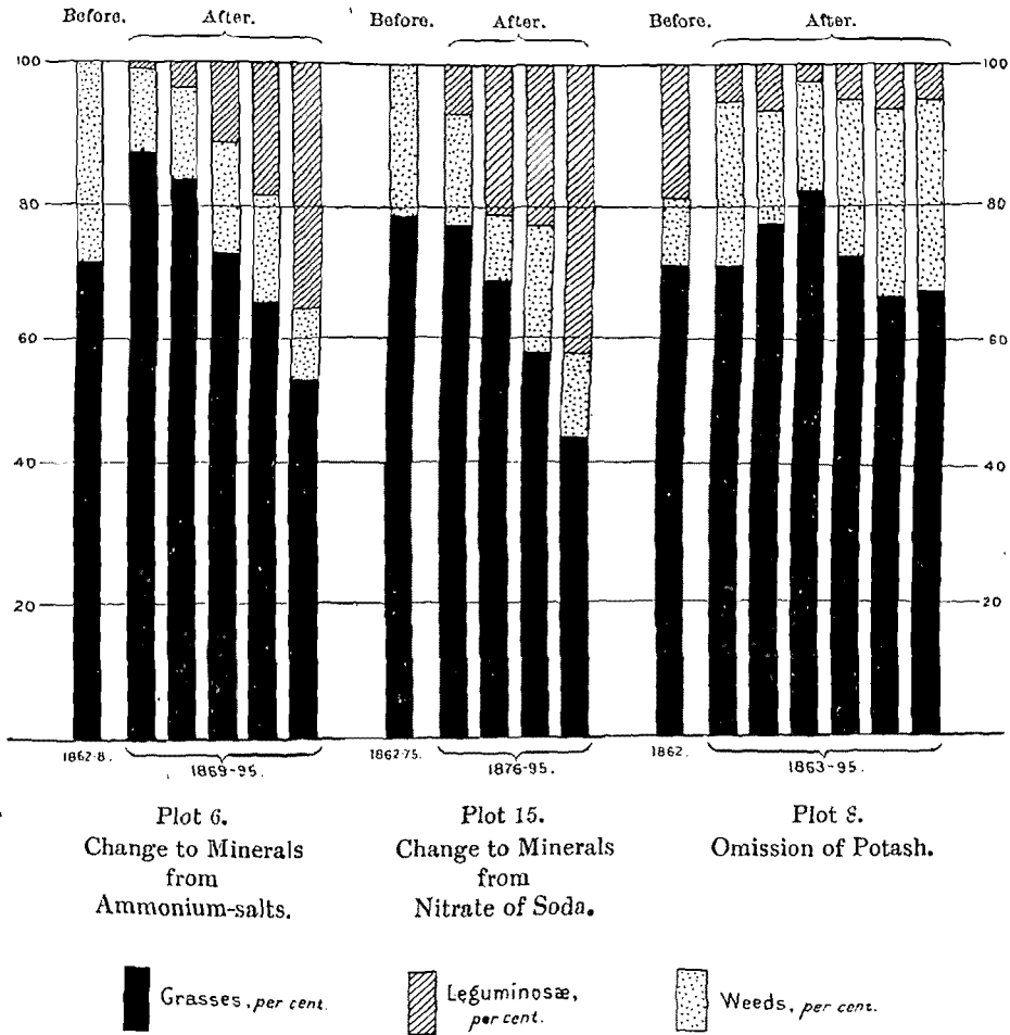
FIG. 29.—Progressive effect of Changes in the Manuring on the Composition of the Hay Crop. Five-year periods.
