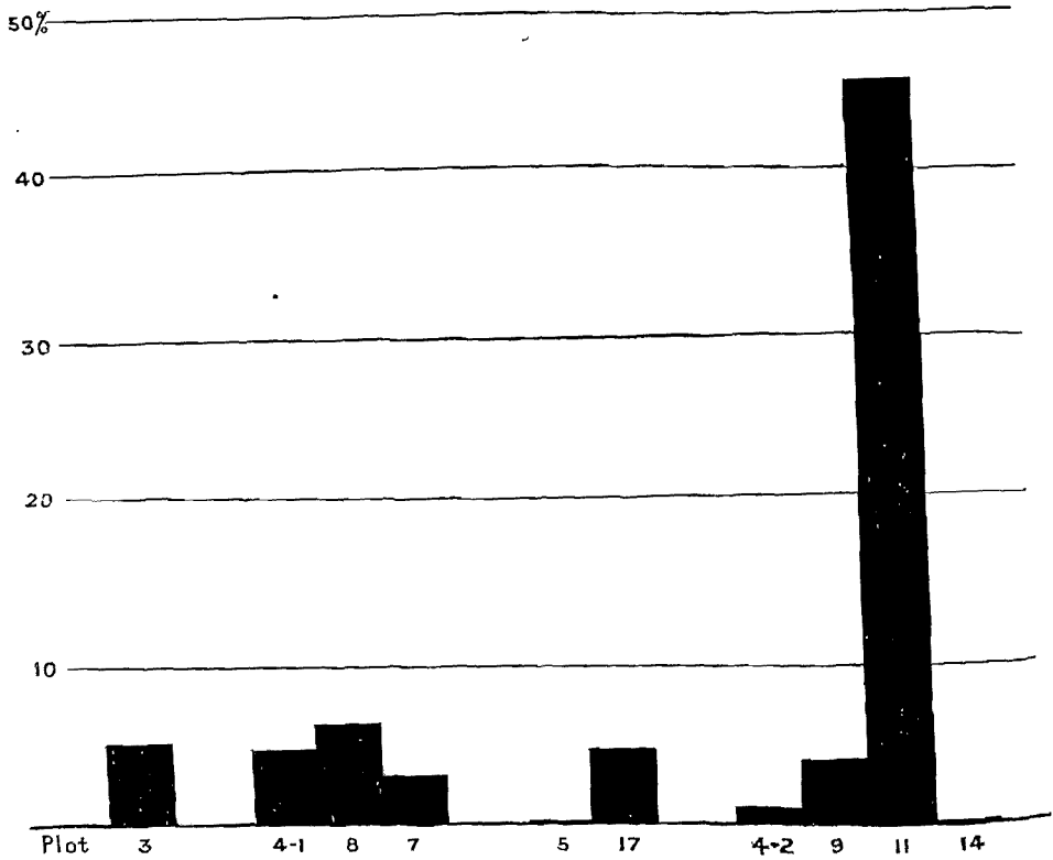
FIG. 38.—Percentage of Holcus lanatus in the Herbage of the Grass Plots. First Crop, Season 1903.
