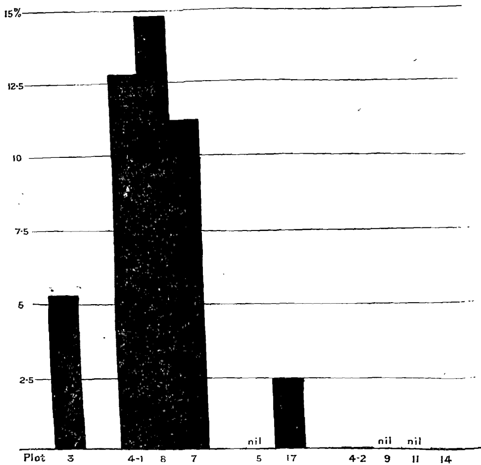
FIG. 37.—Percentage of Trifolium repens , Trifolium pratense , and Lotus corniculatus (together) in the Herbage of the Grass Plots. First Crop, Season 1903.
