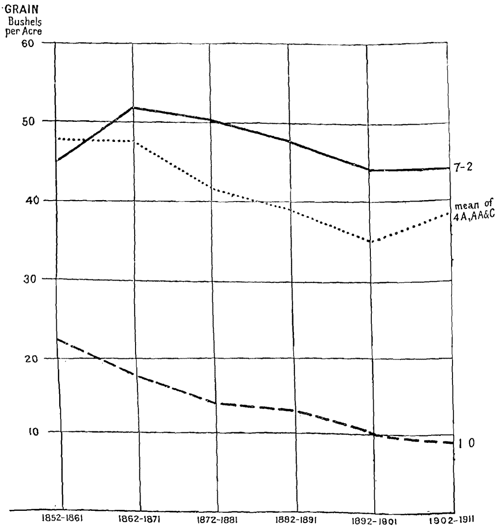
FIG. 10.—Yield of Barley during successive 10-year periods (1852-1911). Plot 7-2.—Farmyard Manure. Plots 4 A, AA, and C.—Each receive Complete Minerals, + N. as Amm.-salts, Nitrate Soda, or Rape Cake. Plot 1 O.—Unmanured.
