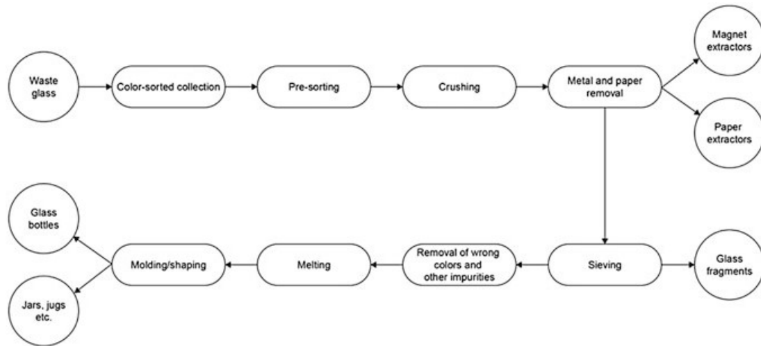
Fig. 3 Glass recycling process (source Arvanitoyannis and Bosnea 2001)
